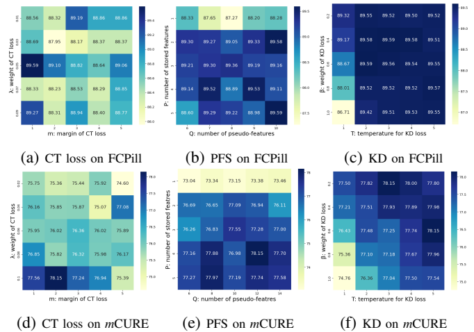
Fig. 9: Hyper-parameter influence on the FCPill and mCURE datasets.
