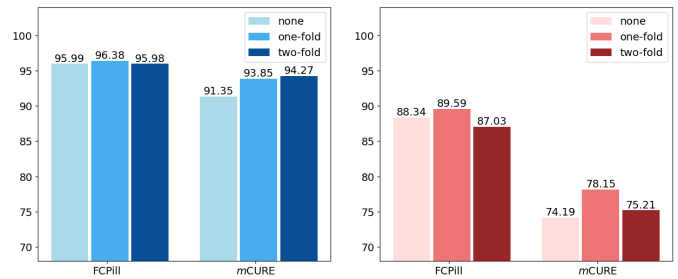
(a) Accuracy on the base session (b) Accuracy on the final session
