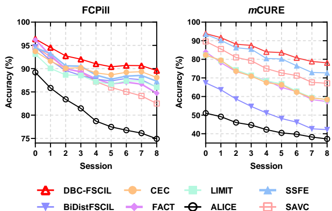
Fig. 4: Comparison with SOTA methods on FCPill and mCURE . Our method, DBC-FSCIL, comprehensively surpasses other methods.
